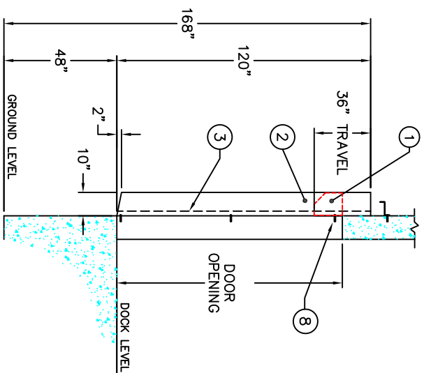
2 STANDARD UNIT DETAIL SIDE VIEW SCALE: 1" = 1'-0"
