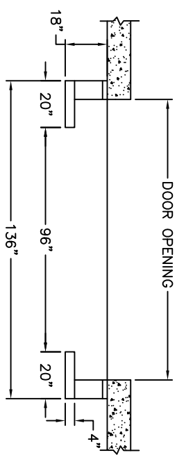
3 STANDARD UNIT DETAIL FLAN VIEW SCALE: 1" = 1'-0"
