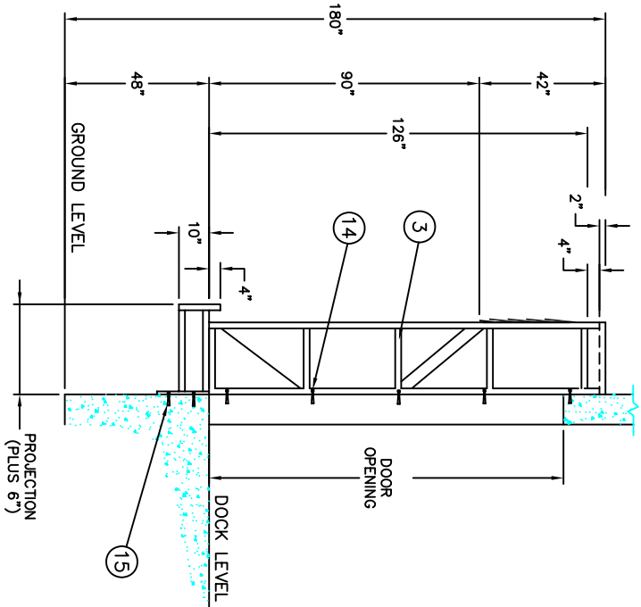
2 STANDARD UNIT DETAIL SIDE VIEW SCALE: 1" = 1'-0"
